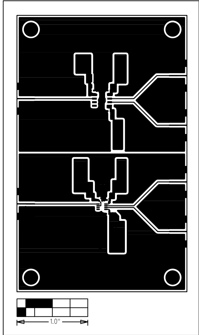
Figure 4. MAX9360 EV Kit PC Board Layout—Component Side
