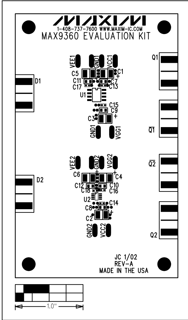
Figure 3. MAX9360 EV Kit Component Placement Guide—Component Side
