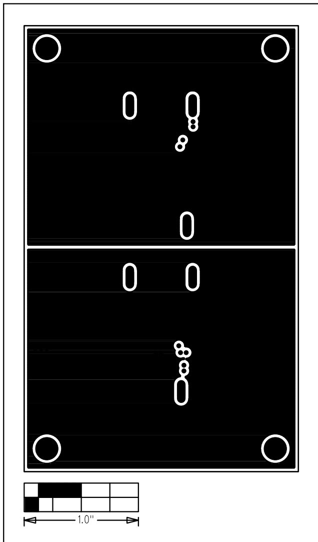
Figure 5. MAX9360 EV Kit PC Board Layout—Inner Layer 2 (Ground Layer)
