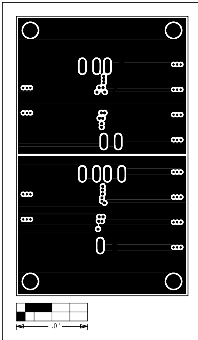
Figure 6. MAX9360 EV Kit PC Board Layout—Inner Layer 3 (VCC Layer)
