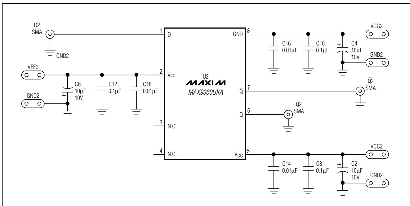
Figure 2. MAX9360 EV Kit Schematic (MAX9360UKA Circuit)
