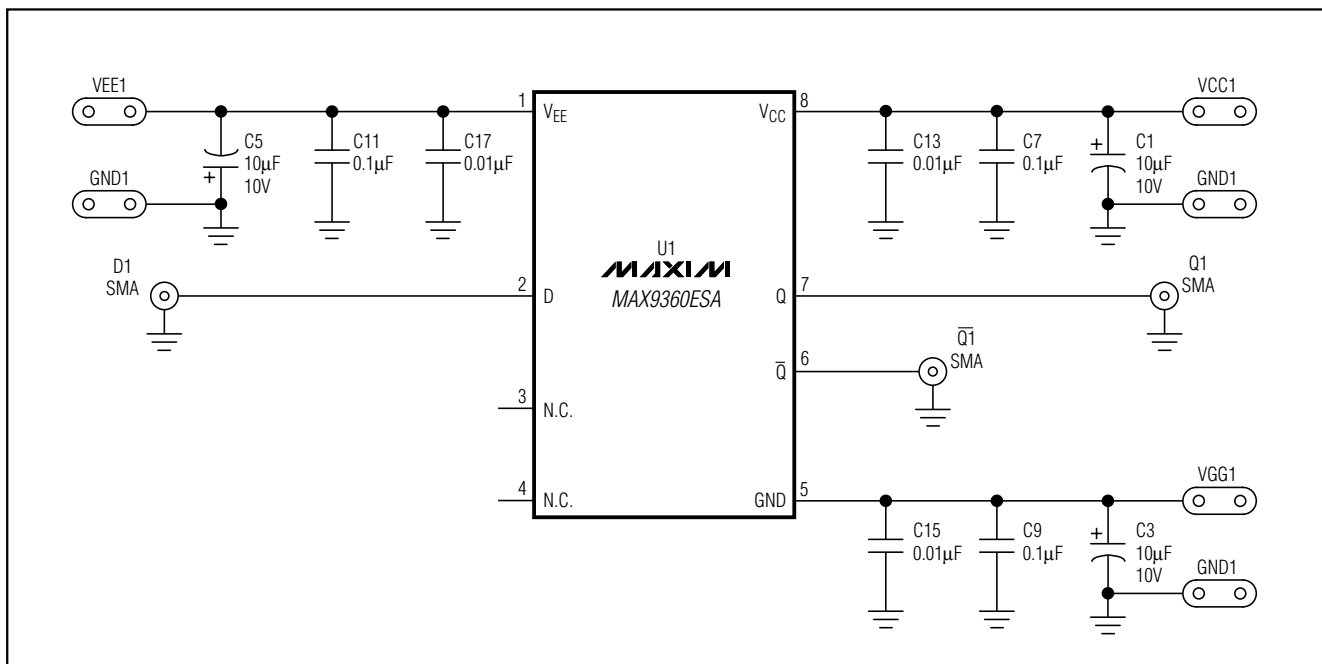
Figure 1. MAX9360 EV Kit Schematic (MAX9360ESA Circuit)
