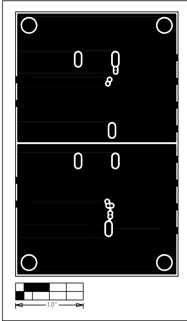
Figure 7. MAX9360 EV Kit PC Board Layout—Solder Side
